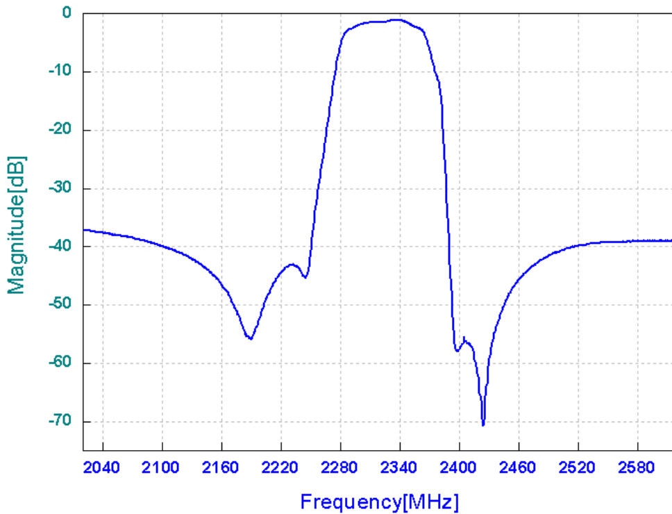
Frequency Response
